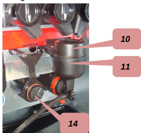
Mengkom detail
